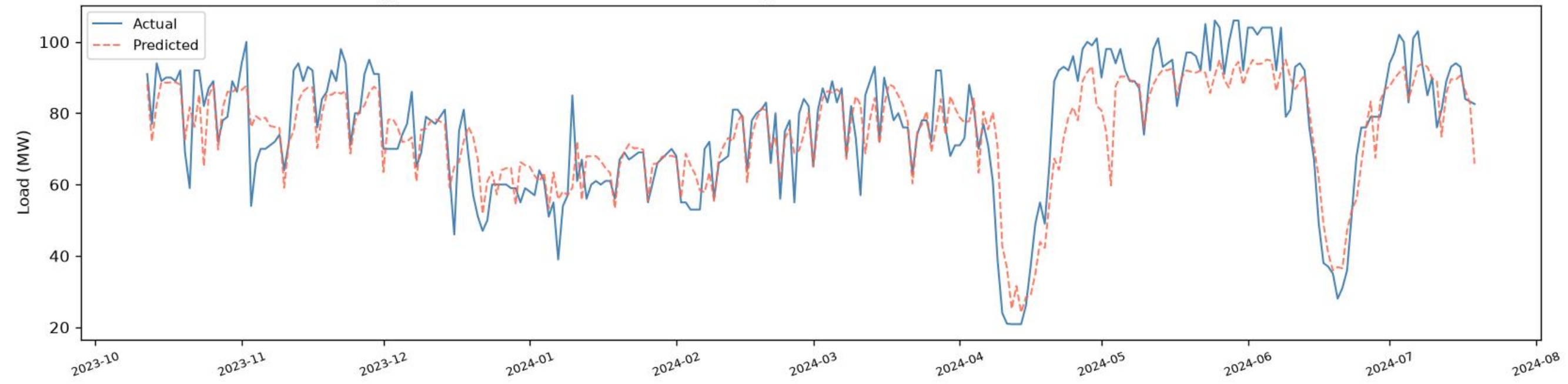
Lalbag | CNN+BiGRU+BiLSTM - VALIDATION (chronological, before test) ( R^2=0.7421 , RMSE=9.18, MAE=6.98, n=272)
