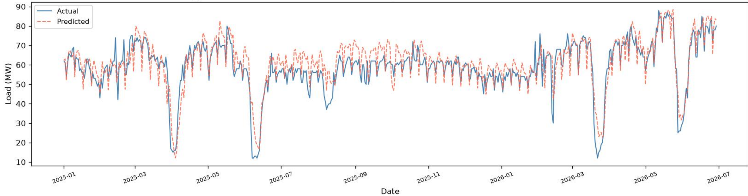
Lalbag | CNN+BiLSTM+BiGRU - TEST ( \geq 2025 ), one-day-ahead ( R^2=0.7534 , RMSE=6.70 , MAE=5.08 , n=527 )
