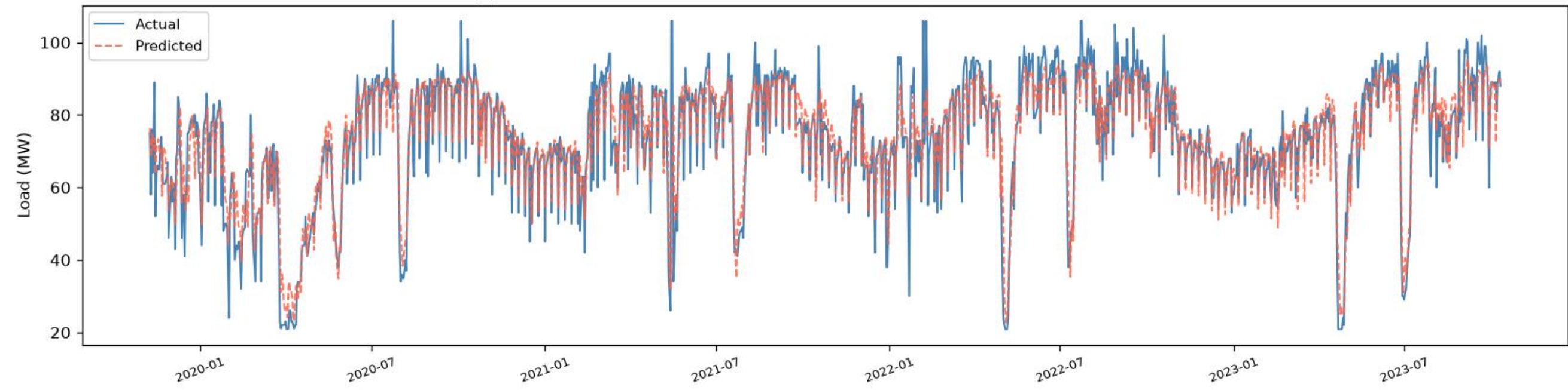
Lalbag | CNN+BiLSTM+BiGRU - TRAIN (fit block) (R2=0.8331, RMSE=6.85, MAE=4.59, n=1398)
