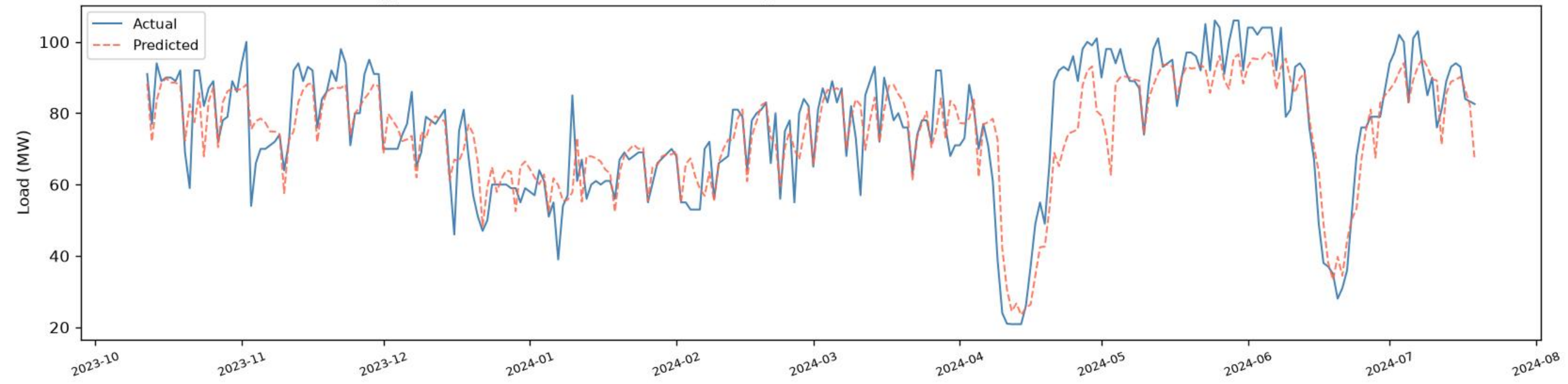
Lalbag | CNN+BiLSTM+BiGRU - VALIDATION (chronological, before test) ( R^2=0.7427 , RMSE=9.17, MAE=6.82, n=272 )
