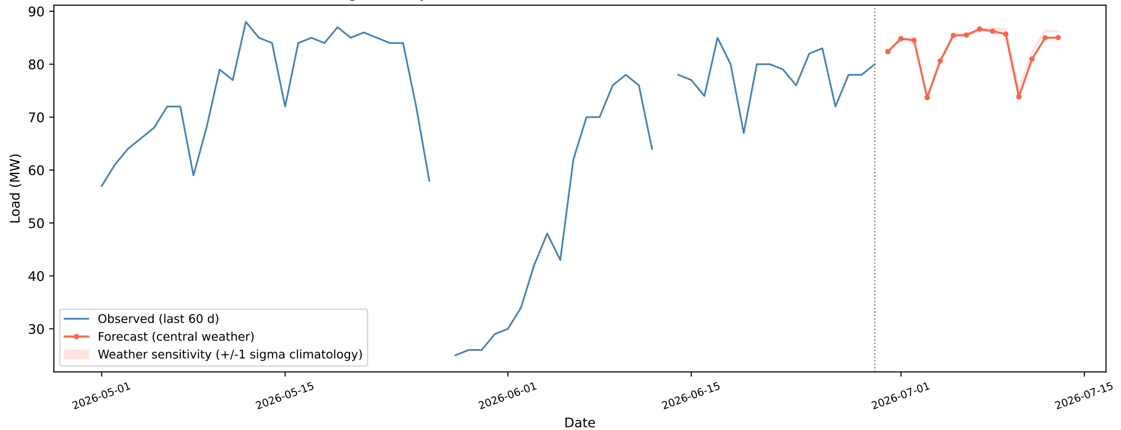
Lalbag - 14-day recursive forecast (BiGRU), weather mode = forecast
