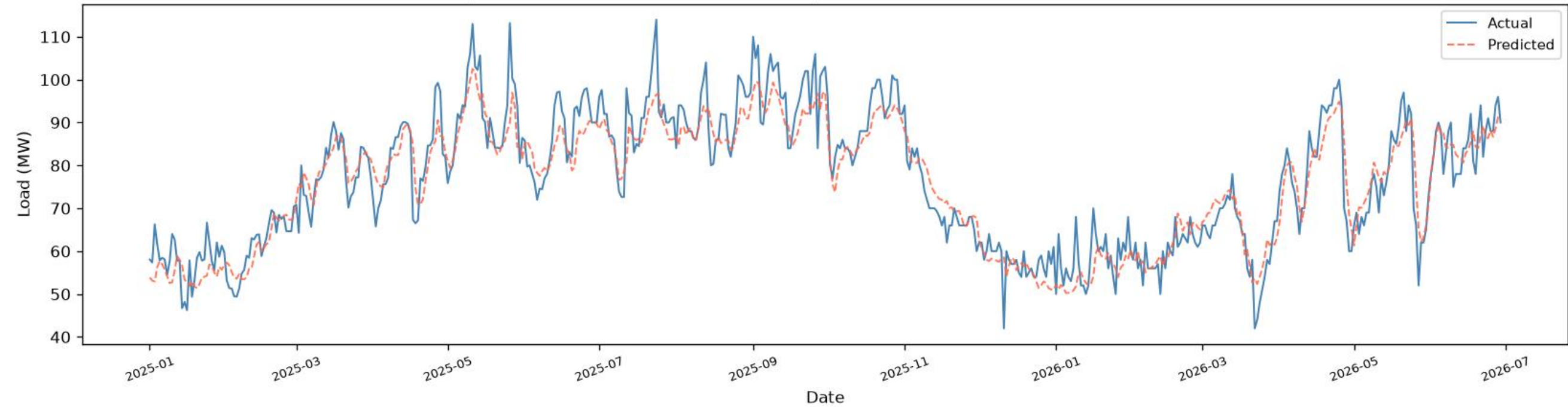
Madartek | BiGRU+BiLSTM - TEST ( \geq 2025 ), one-day-ahead ( R^2=0.8785 , RMSE=5.45 , MAE=4.26 , n=528 )
