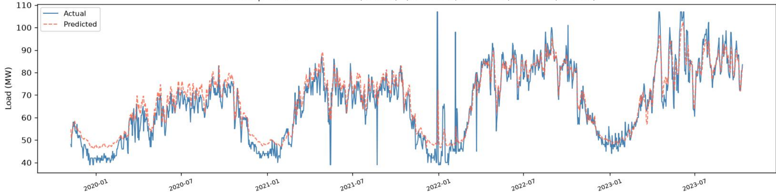
Madartek | BiGRU+BiLSTM - TRAIN (fit block) (R2=0.8734, RMSE=5.52, MAE=3.94, n=1394)
