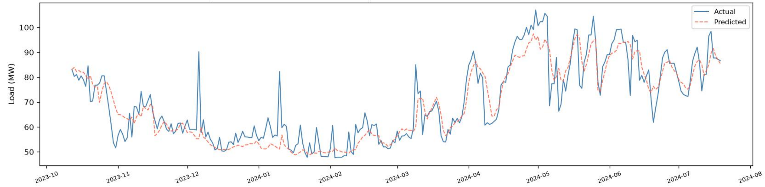
Madartek | BiGRU+BiLSTM - VALIDATION (chronological, before test) ( R^2=0.8156 , RMSE=6.76, MAE=4.74, n=272 )
