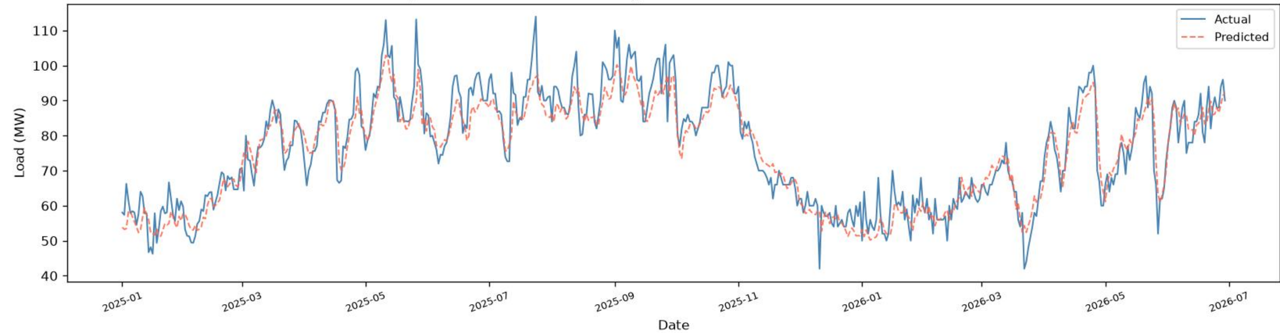
Madartek | BiGRU - TEST ( \geq 2025 ), one-day-ahead ( R^2=0.8832 , RMSE=5.35 , MAE=4.14 , n=528 )
