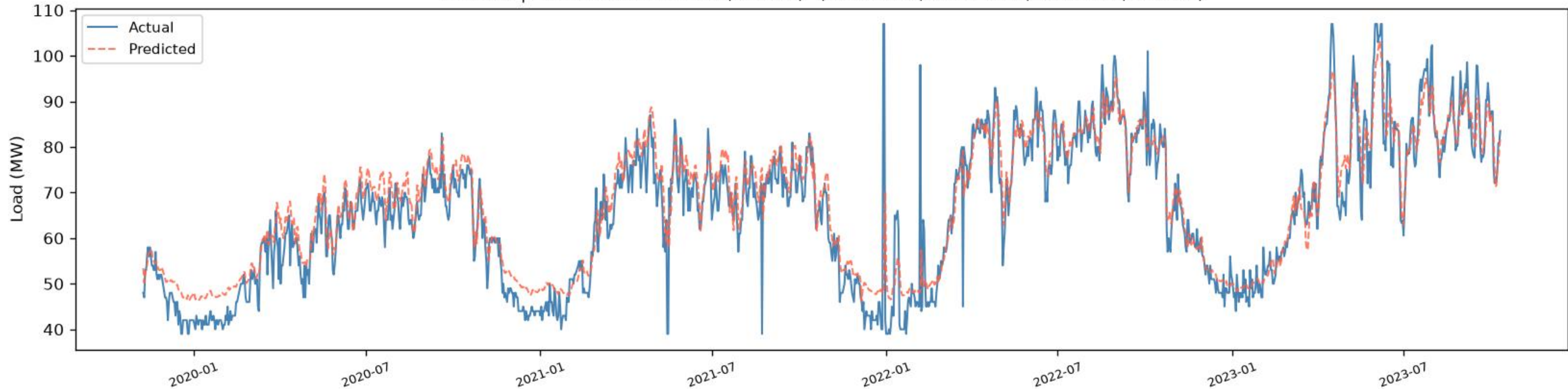
Madartek | BiLSTM+BiGRU - TRAIN (fit block) (R2=0.8782, RMSE=5.42, MAE=3.81, n=1394)
