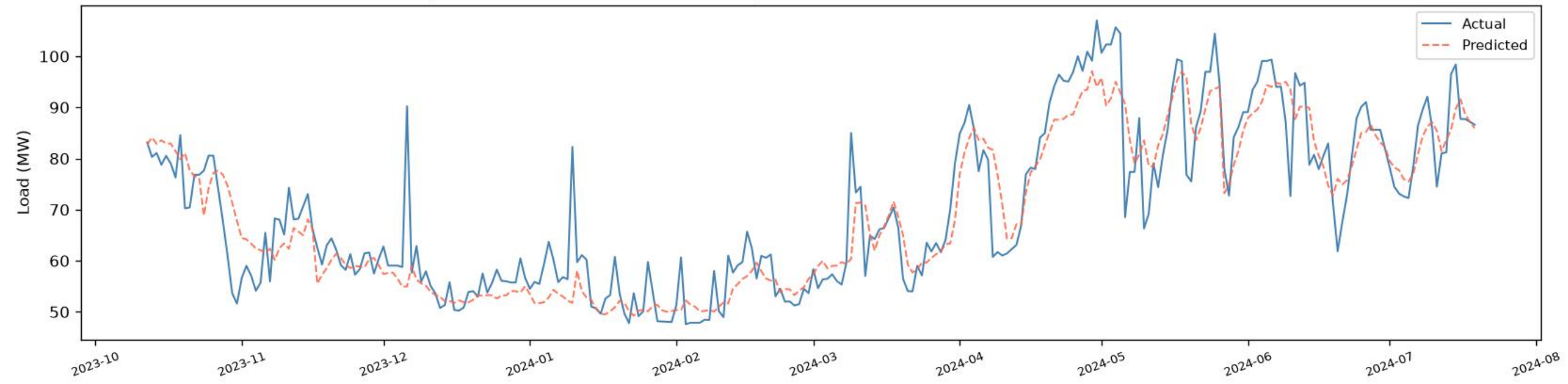
Madartek | BiLSTM+BiGRU - VALIDATION (chronological, before test) ( R^2=0.8110 , RMSE=6.84 , MAE=4.87 , n=272 )
