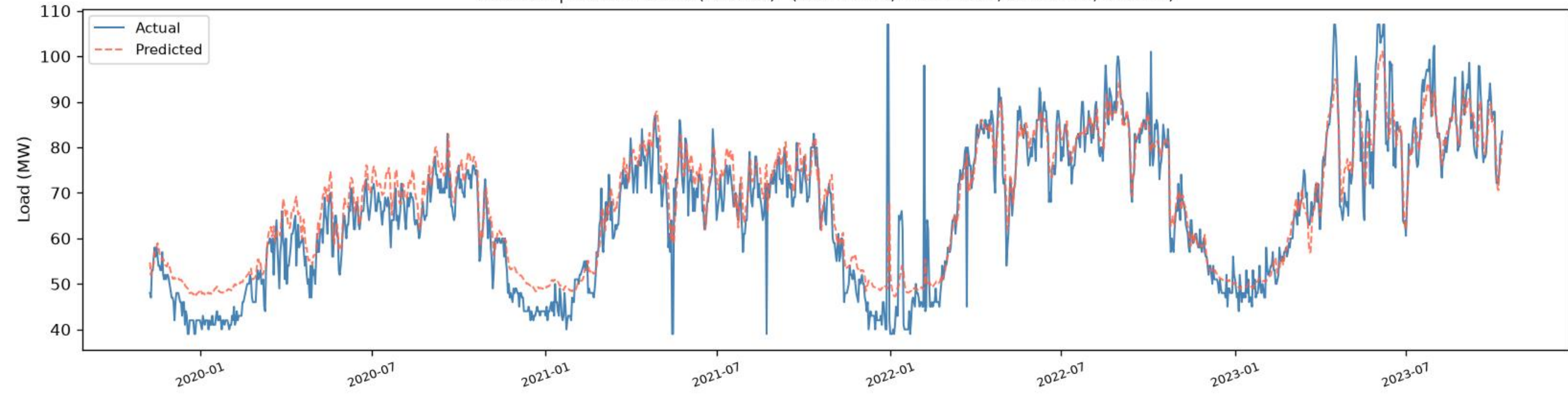
Madartek | BiLSTM - TRAIN (fit block) (R2=0.8668, RMSE=5.66, MAE=4.09, n=1394)
