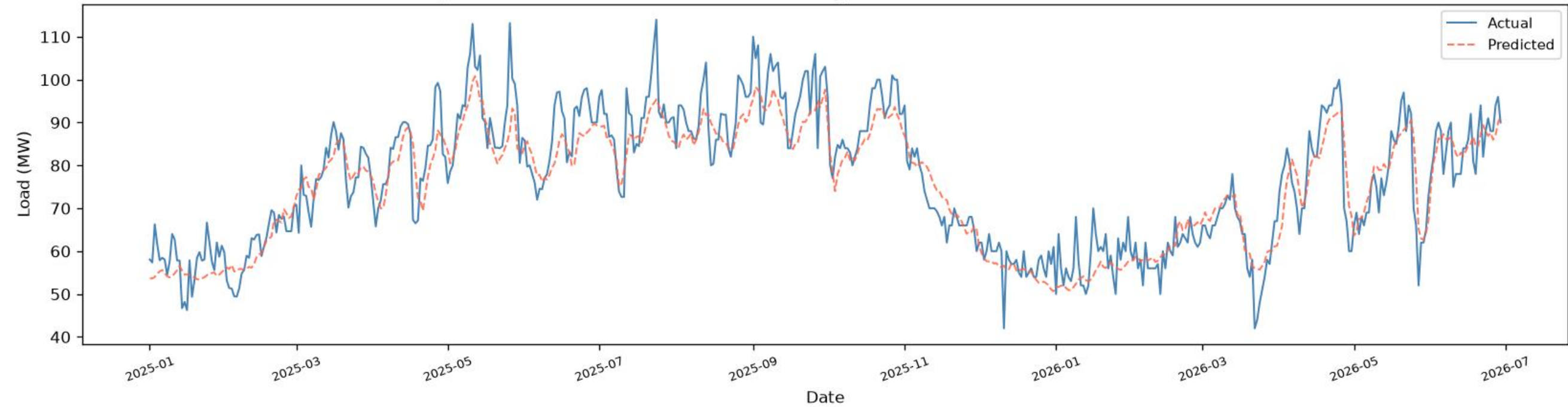
Madartek | CNN+BiGRU+BiLSTM - TEST ( \geq 2025 ), one-day-ahead ( R^2=0.8588 , RMSE=5.88 , MAE=4.62 , n=528 )
