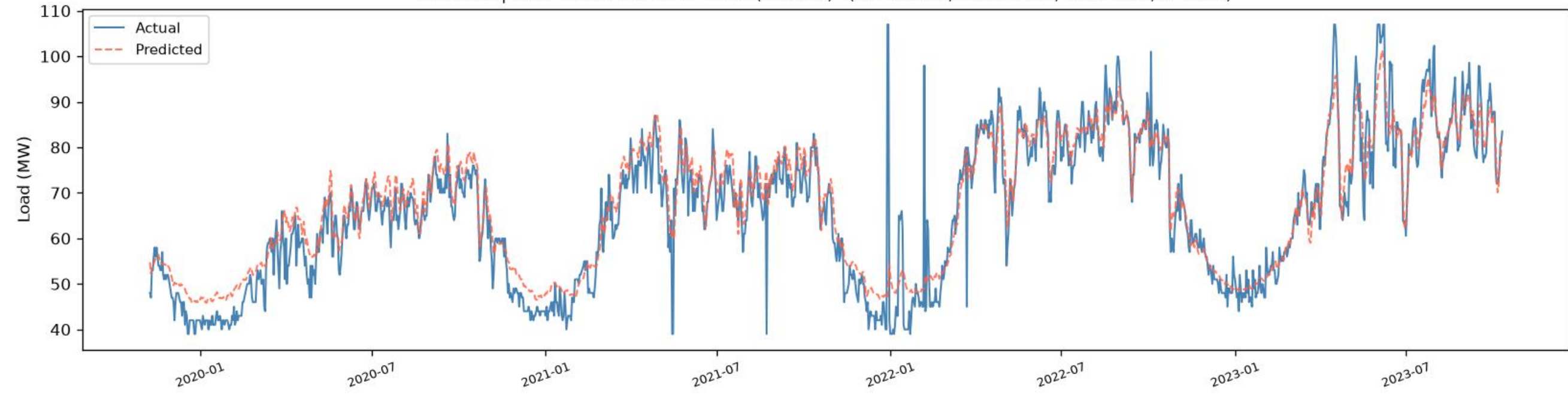
Madartek | CNN+BiGRU+BiLSTM - TRAIN (fit block) (R2=0.8777, RMSE=5.43, MAE=3.76, n=1394)
