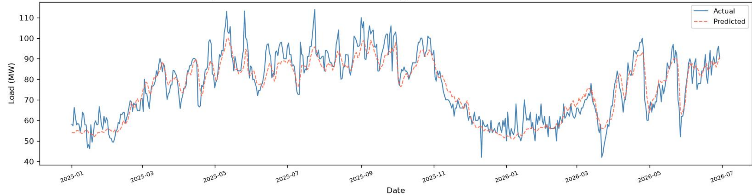
Madartek | CNN+BiLSTM+BiGRU - TEST ( \geq 2025 ), one-day-ahead ( R^2=0.8619 , RMSE=5.81 , MAE=4.61 , n=528 )
