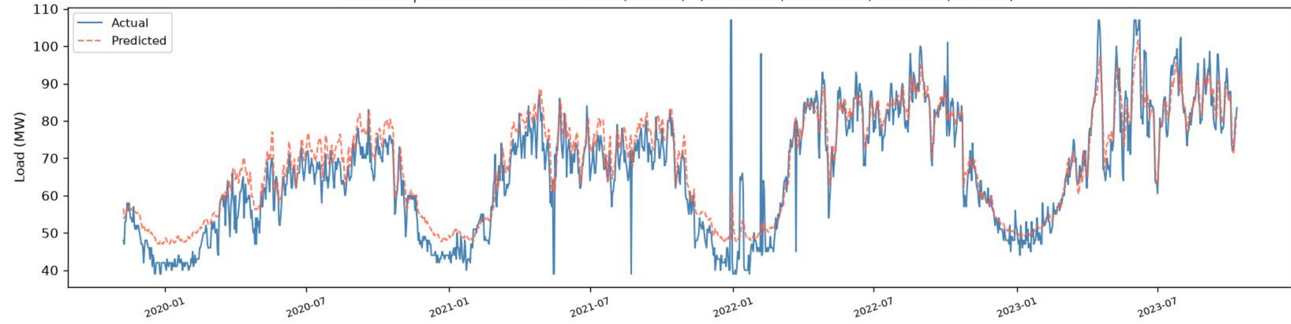
Madartek | CNN+BiLSTM+BiGRU - TRAIN (fit block) (R2=0.8558, RMSE=5.90, MAE=4.32, n=1394)
