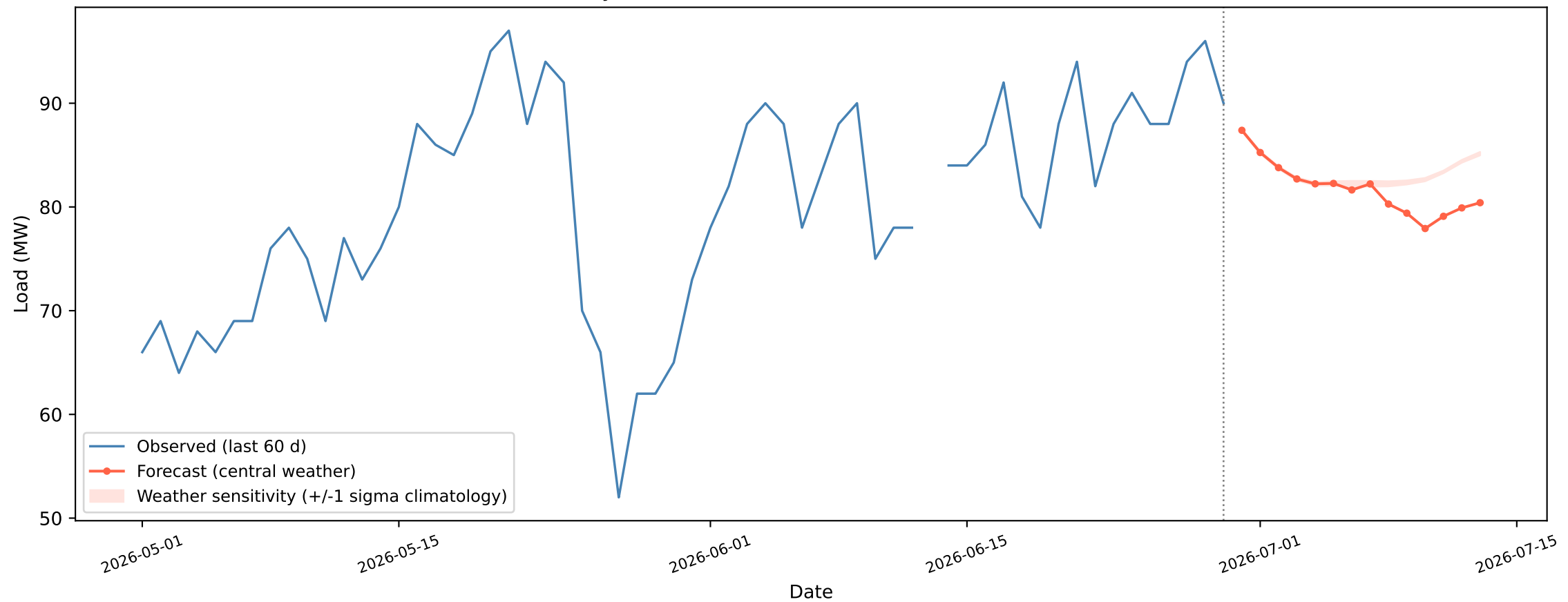
Madartek - 14-day recursive forecast (BiGRU), weather mode = forecast
