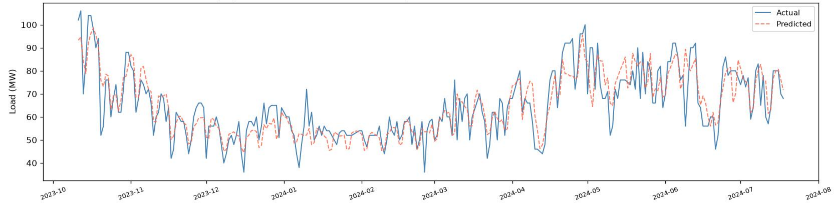
Maniknagar | BiGRU+BiLSTM - VALIDATION (chronological, before test) ( R^2=0.7291 , RMSE=7.48 , MAE=5.56 , n=271 )
