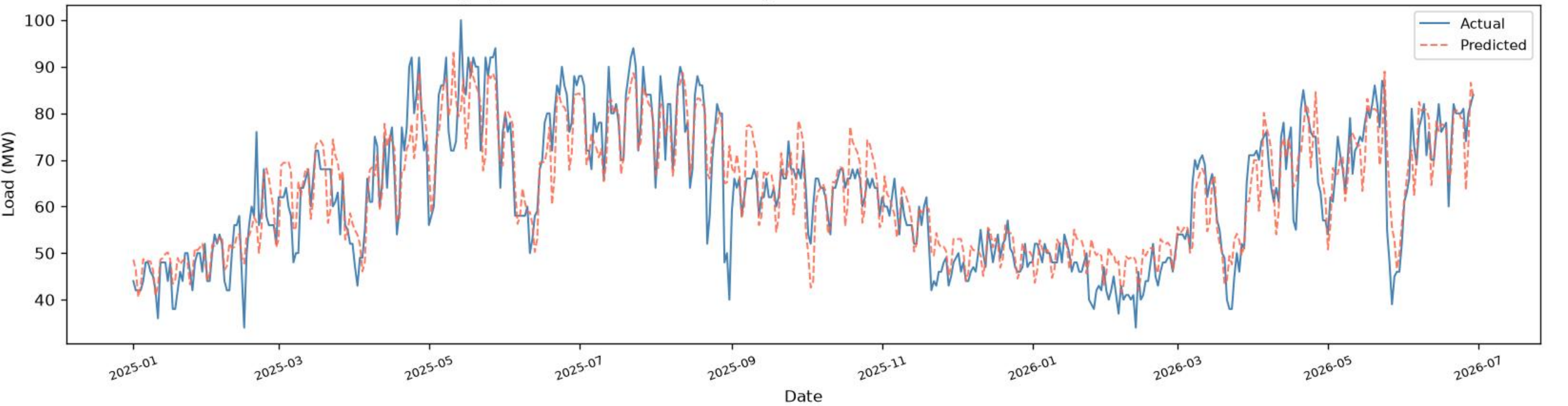
Maniknagar | BiGRU - TEST ( \geq 2025 ), one-day-ahead ( R^2=0.8169 , RMSE=6.18 , MAE=4.73 , n=525 )
