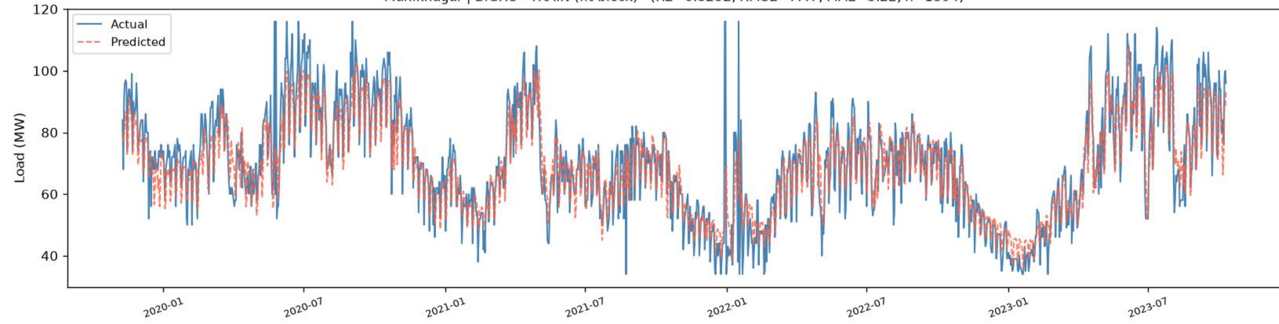
Maniknagar | BiGRU - TRAIN (fit block) ( R^2=0.8232 , RMSE=7.47, MAE=5.22, n=1394)
