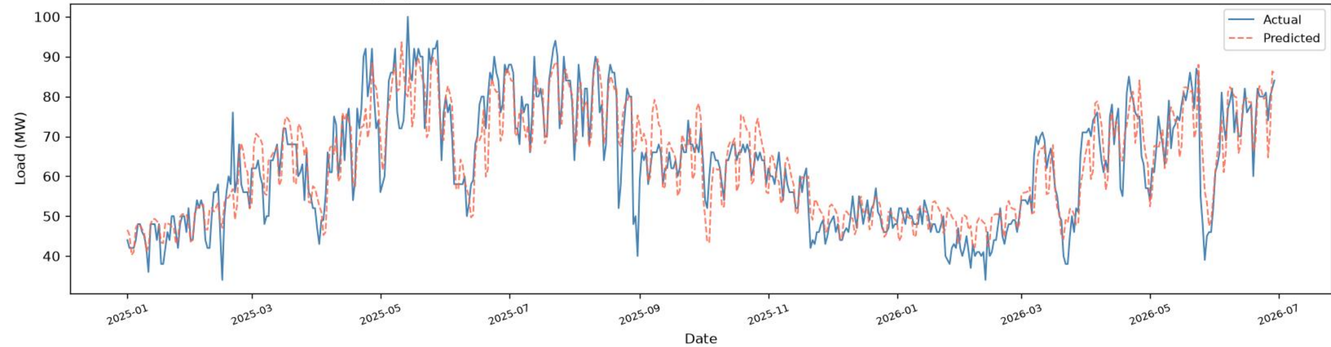
Maniknagar | BiLSTM+BiGRU - TEST ( \geq 2025 ), one-day-ahead ( R^2=0.8022 , RMSE=6.43 , MAE=4.89 , n=525 )
