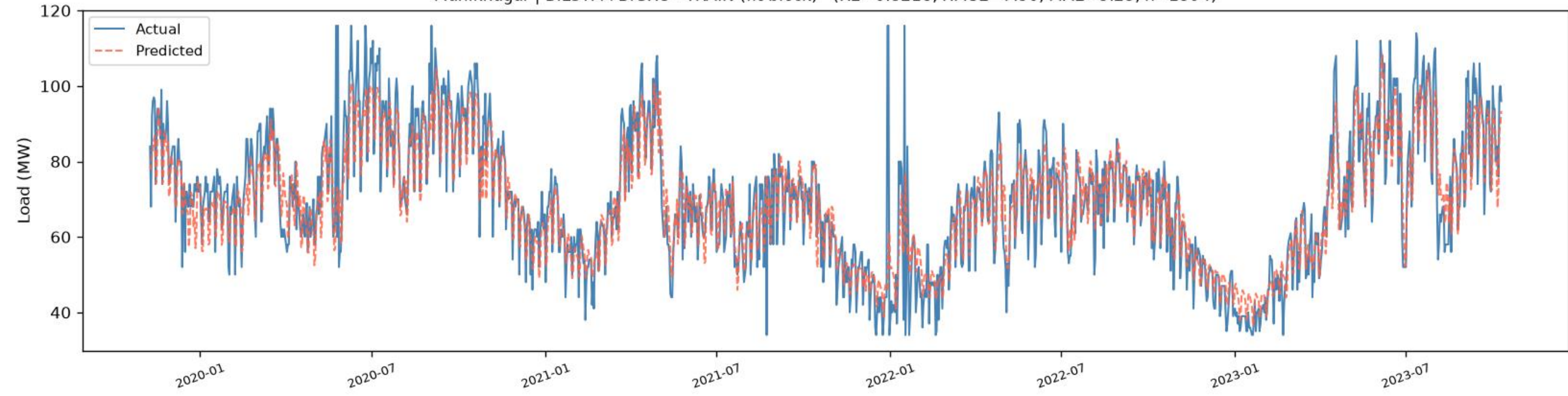
Maniknagar | BiLSTM+BiGRU - TRAIN (fit block) (R2=0.8218, RMSE=7.50, MAE=5.25, n=1394)
