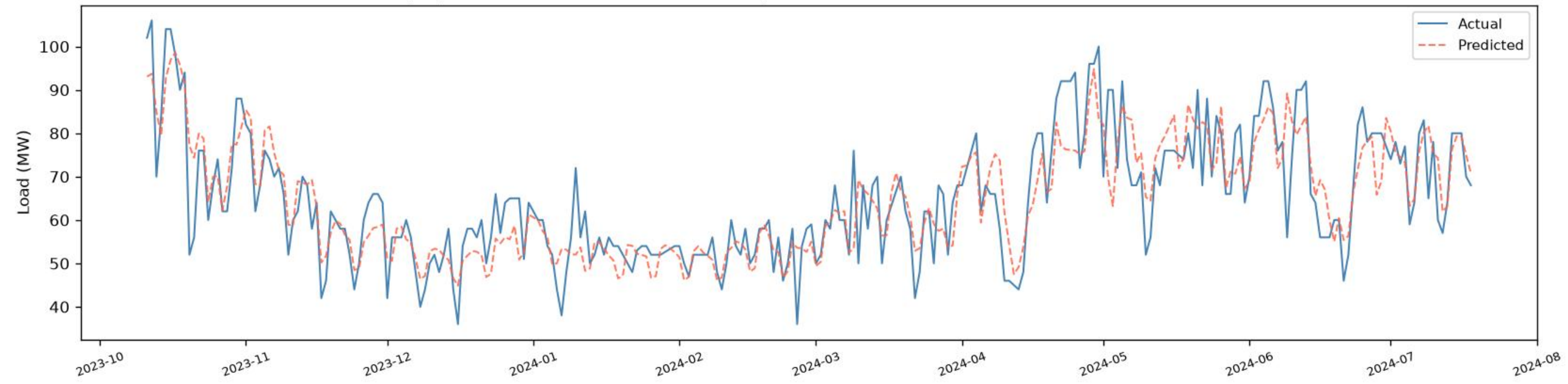
Maniknagar | BiLSTM+BiGRU - VALIDATION (chronological, before test) ( R^2=0.7151 , RMSE=7.67 , MAE=5.74 , n=271 )
