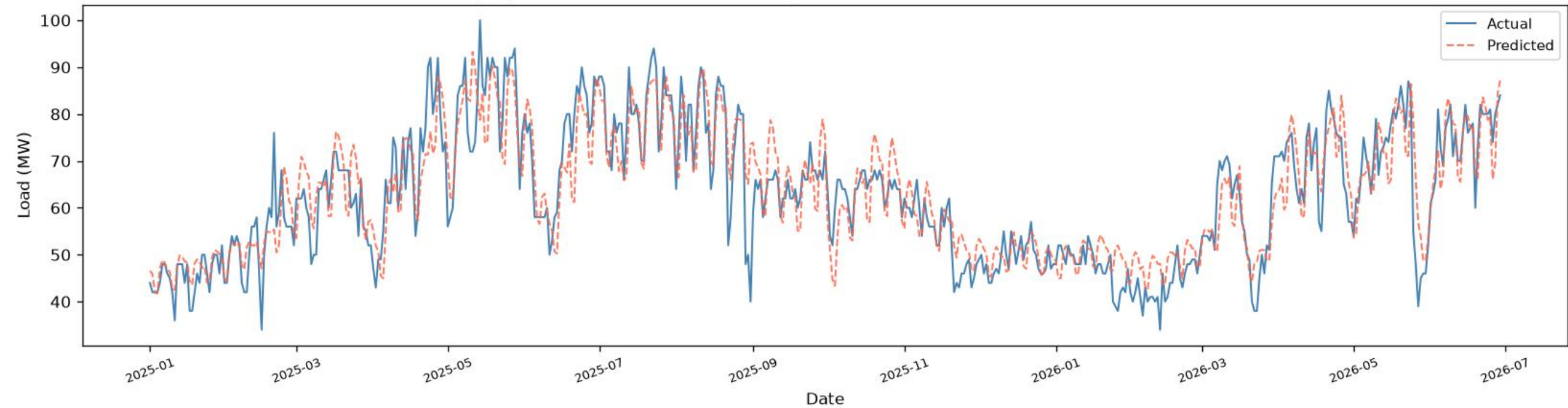
Maniknagar | BiLSTM - TEST ( \geq 2025 ), one-day-ahead ( R^2=0.7895 , RMSE=6.63 , MAE=5.05 , n=525 )
