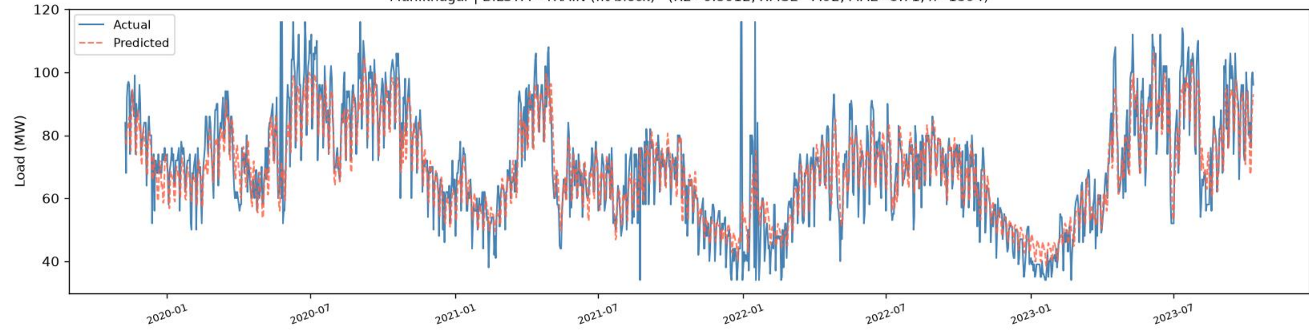
Maniknagar | BiLSTM - TRAIN (fit block) ( R^2=0.8012 , RMSE=7.92, MAE=5.71, n=1394)
