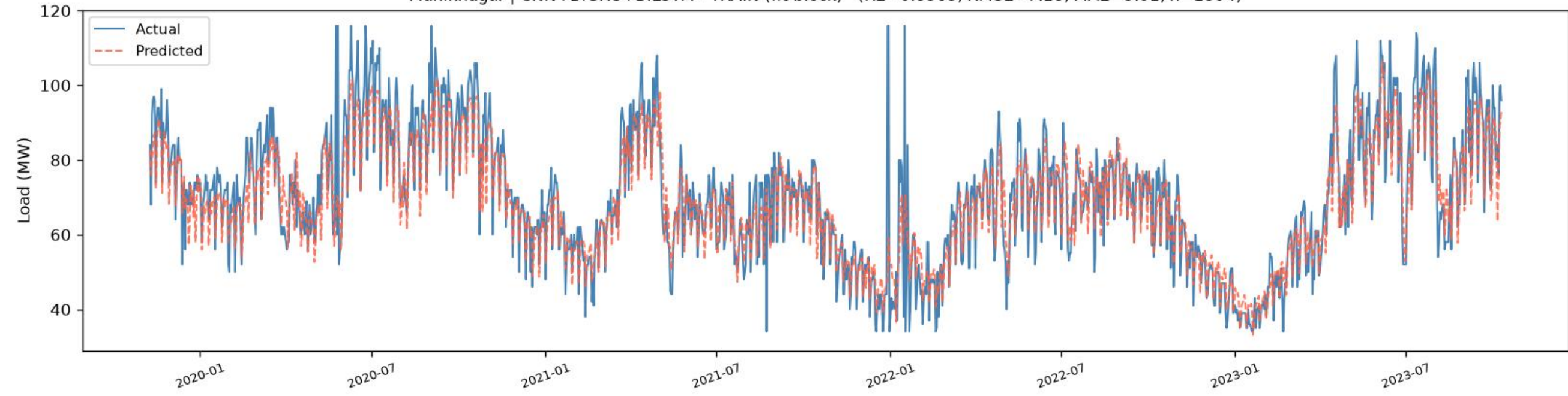
Maniknagar | CNN+BiGRU+BiLSTM - TRAIN (fit block) (R2=0.8365, RMSE=7.18, MAE=5.01, n=1394)
