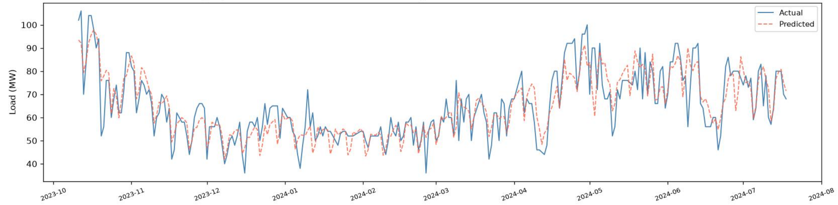
Maniknagar | CNN+BiGRU+BiLSTM - VALIDATION (chronological, before test) ( R^2=0.7249 , RMSE=7.54 , MAE=5.51 , n=271 )
