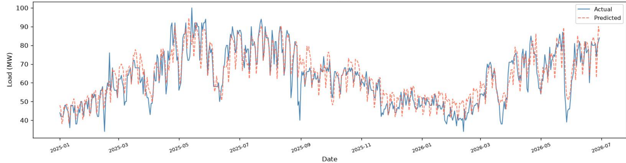
Maniknagar | CNN+BiLSTM+BiGRU - TEST ( \geq 2025 ), one-day-ahead ( R^2=0.8051 , RMSE=6.38 , MAE=4.94 , n=525 )
