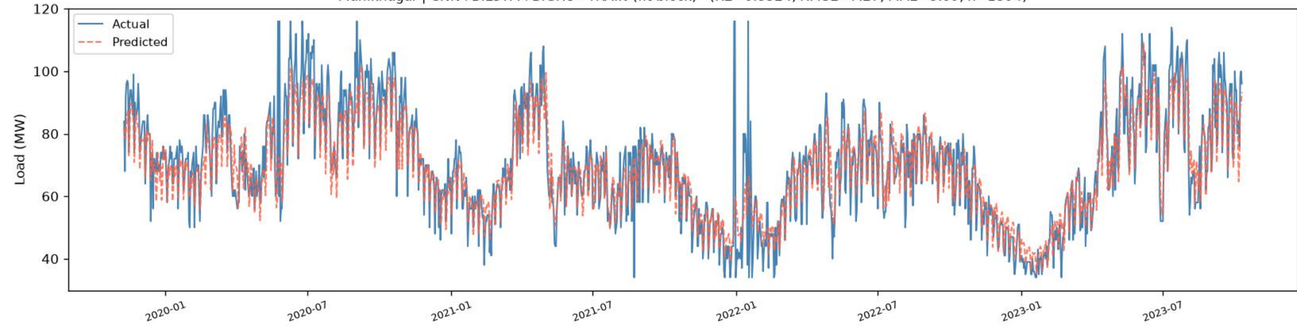
Maniknagar | CNN+BiLSTM+BiGRU - TRAIN (fit block) (R2=0.8324, RMSE=7.27, MAE=5.09, n=1394)
