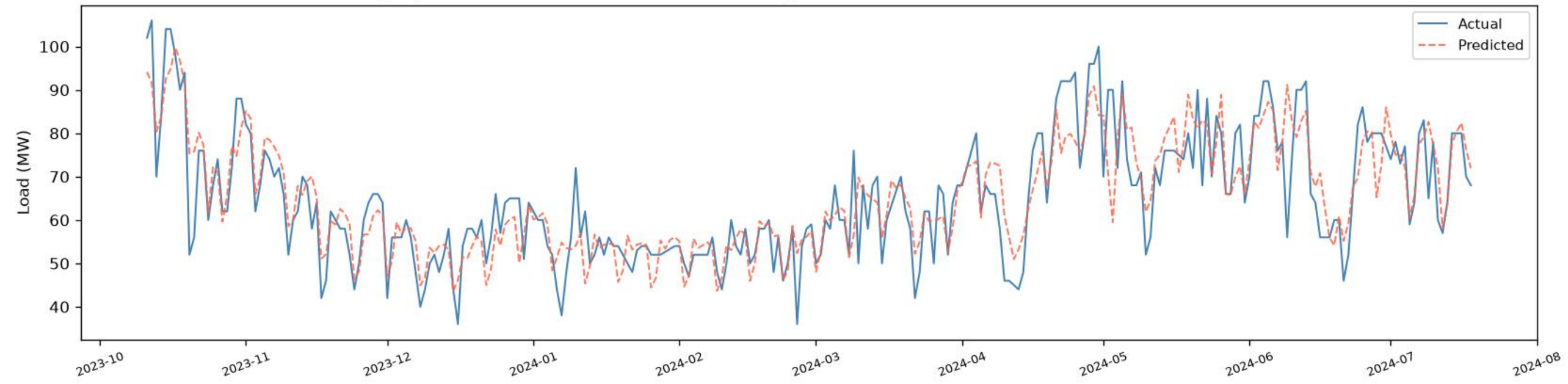
Maniknagar | CNN+BiLSTM+BiGRU - VALIDATION (chronological, before test) ( R^2=0.7312 , RMSE=7.45 , MAE=5.43 , n=271 )
