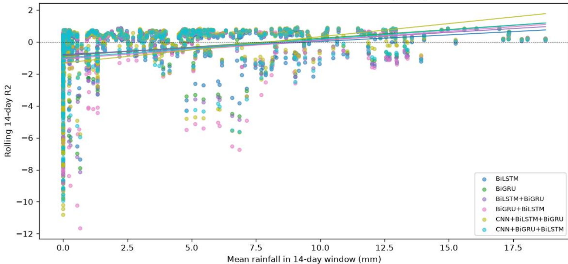
Maniknagar - Rain vs R2 (all 6 models, test period)
