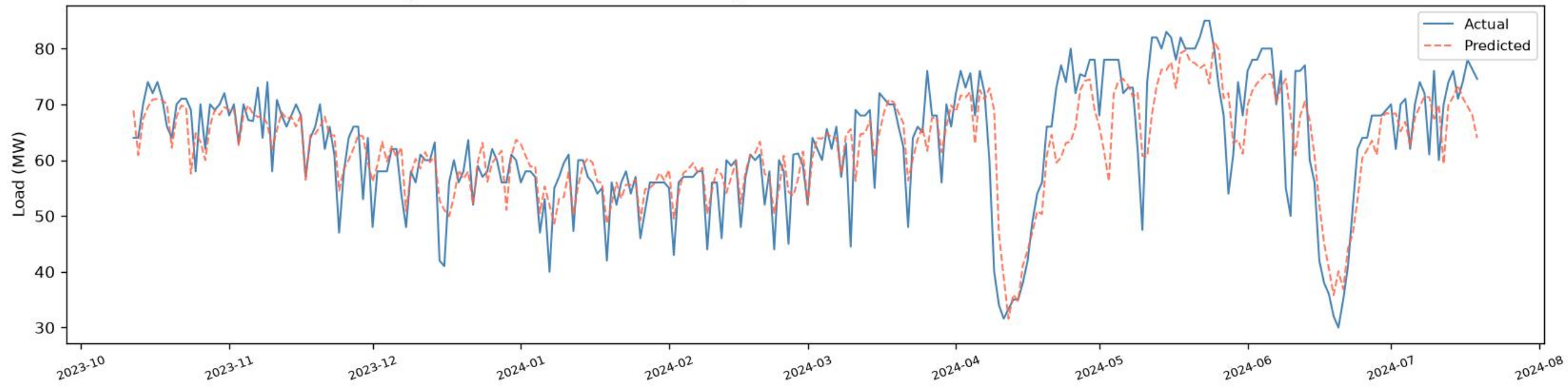
Matual | BiGRU+BiLSTM - VALIDATION (chronological, before test) ( R^2=0.6863 , RMSE=6.31 , MAE=4.58 , n=272 )
