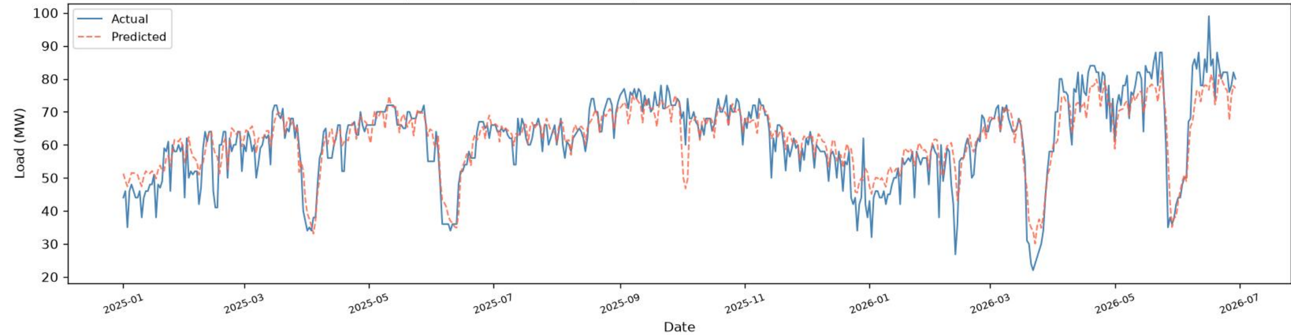
Matual | BiGRU - TEST ( \geq 2025 ), one-day-ahead ( R^2=0.8118 , RMSE=5.63 , MAE=4.16 , n=499 )
