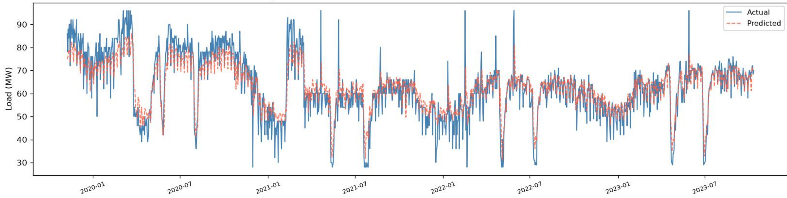
Matual | BiGRU - TRAIN (fit block) ( R^2=0.7832 , RMSE=6.32, MAE=4.60, n=1398 )
