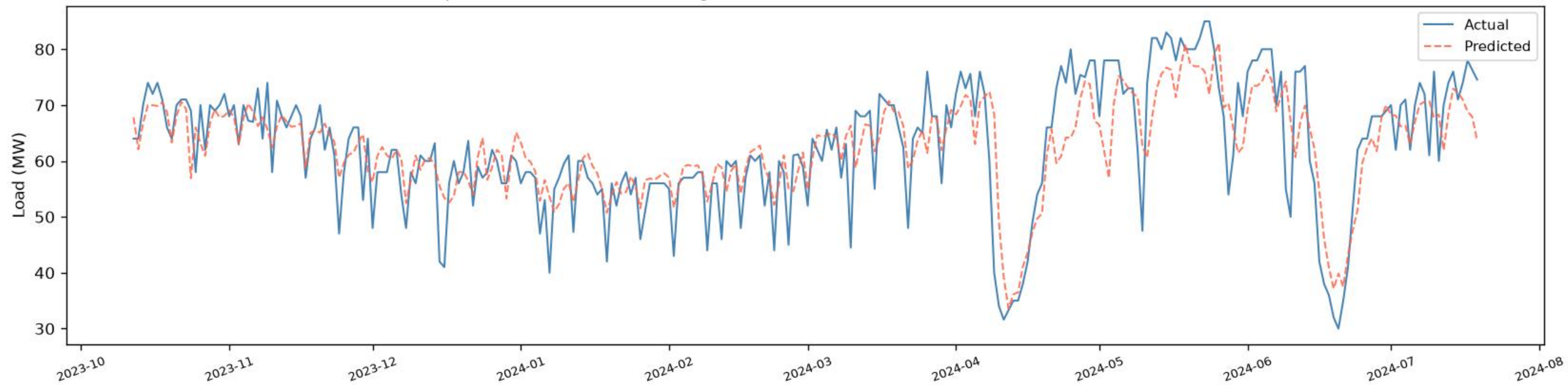
Matual | BiGRU - VALIDATION (chronological, before test) (R2=0.6608, RMSE=6.56, MAE=4.87, n=272)
