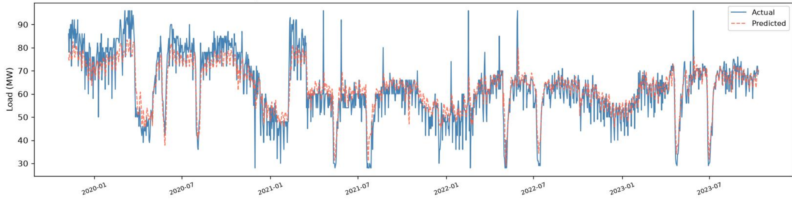
Matual | BiLSTM+BiGRU - TRAIN (fit block) ( R^2=0.7672 , RMSE=6.55 , MAE=4.88 , n=1398 )
