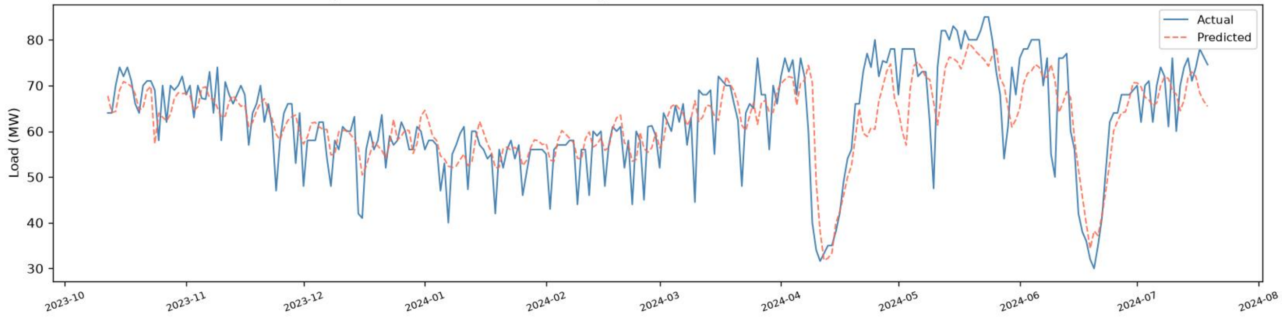
Matual | BiLSTM+BiGRU - VALIDATION (chronological, before test) (R2=0.6289, RMSE=6.86, MAE=5.07, n=272)
