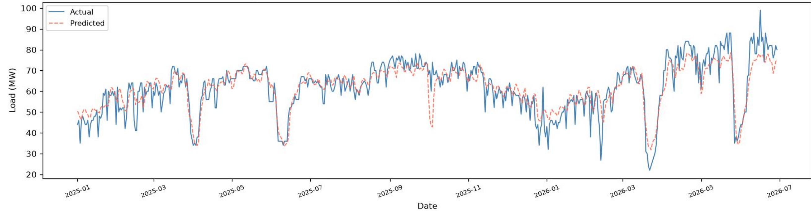
Matual | BiLSTM - TEST ( \geq 2025 ), one-day-ahead ( R^2=0.7819 , RMSE=6.06 , MAE=4.55 , n=499 )
