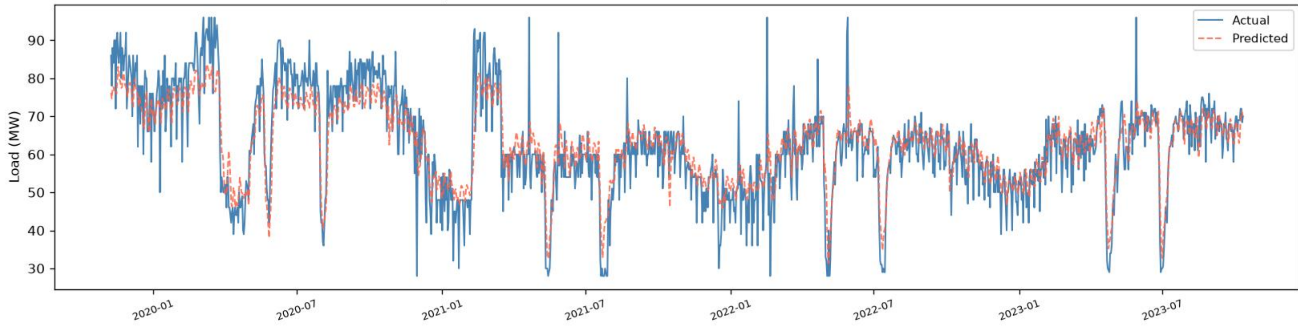
Matual | BiLSTM - TRAIN (fit block) ( R^2=0.7616 , RMSE=6.63, MAE=4.93, n=1398)
