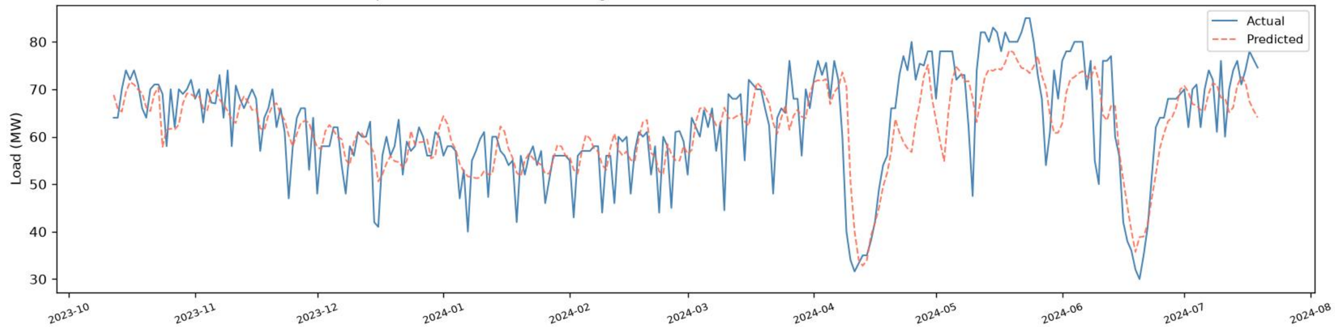
Matual | BiLSTM - VALIDATION (chronological, before test) (R2=0.5866, RMSE=7.24, MAE=5.40, n=272)
