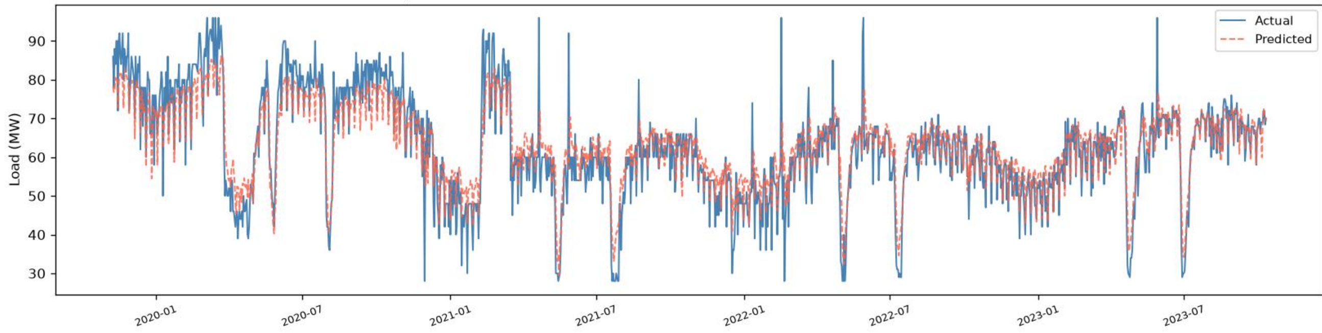
Matual | CNN+BiGRU+BiLSTM - TRAIN (fit block) (R2=0.8021, RMSE=6.04, MAE=4.47, n=1398)
