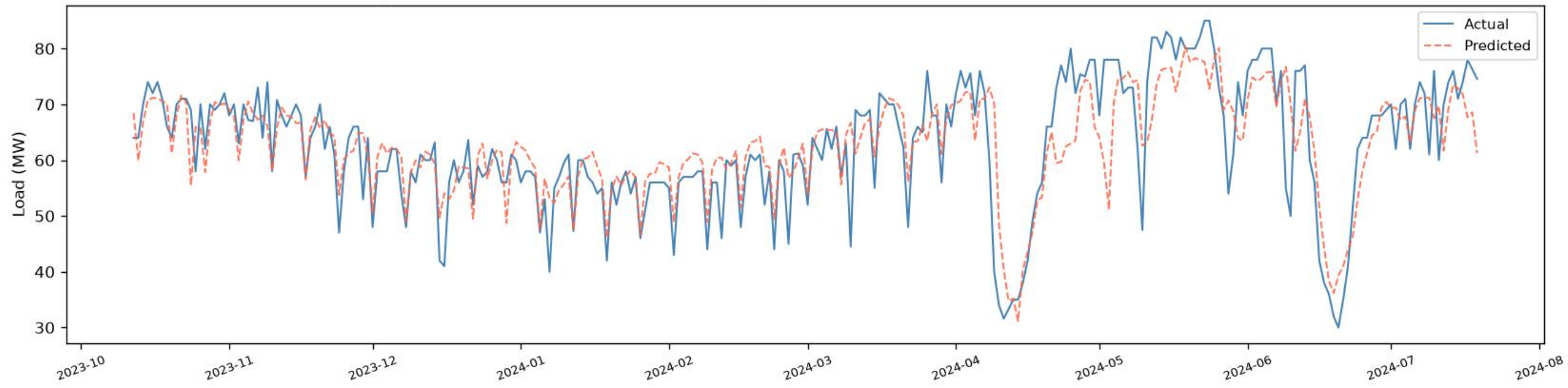
Matual | CNN+BiGRU+BiLSTM - VALIDATION (chronological, before test) (R2=0.6650, RMSE=6.52, MAE=4.63, n=272)
