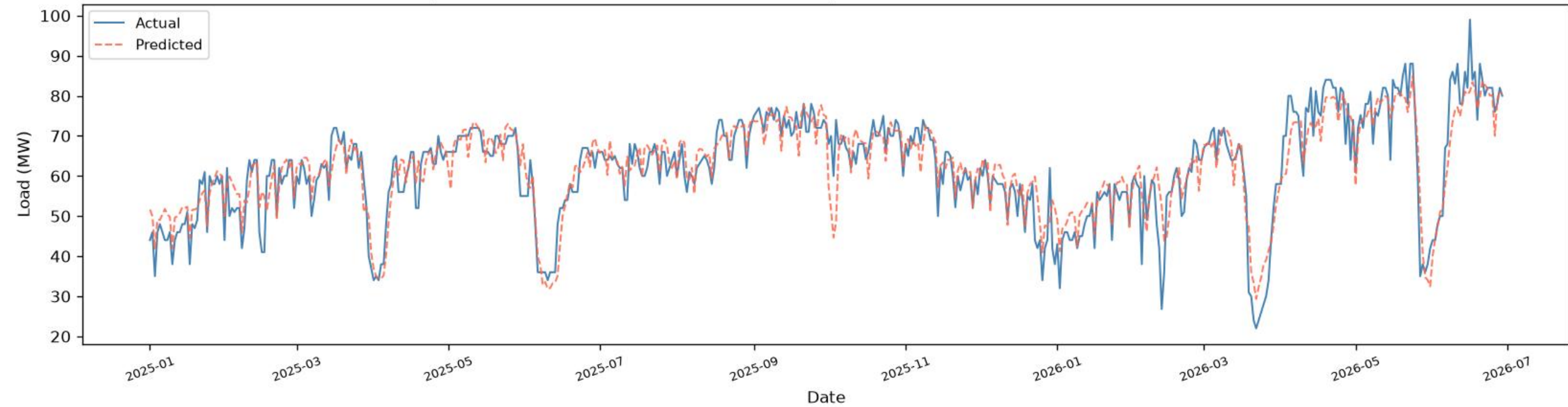
Matual | CNN+BiLSTM+BiGRU - TEST ( \geq 2025 ), one-day-ahead ( R^2=0.8342 , RMSE=5.29 , MAE=3.89 , n=499 )
