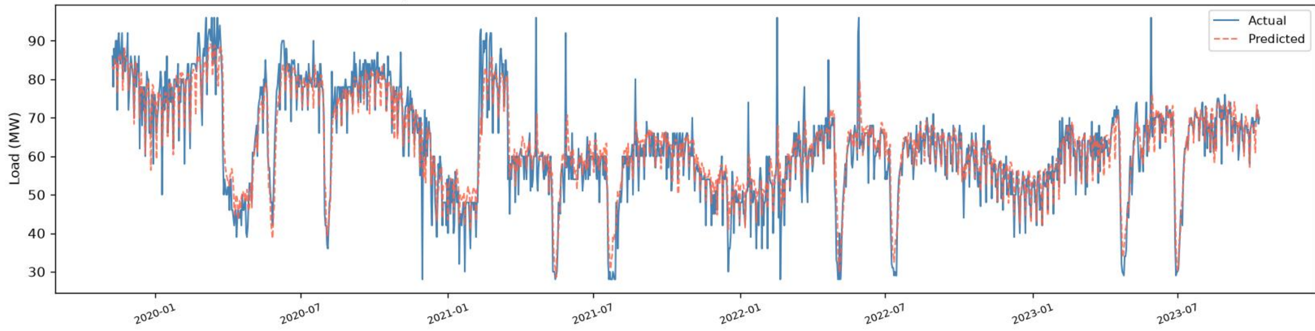
Matual | CNN+BiLSTM+BiGRU - TRAIN (fit block) (R2=0.8436, RMSE=5.37, MAE=3.76, n=1398)
