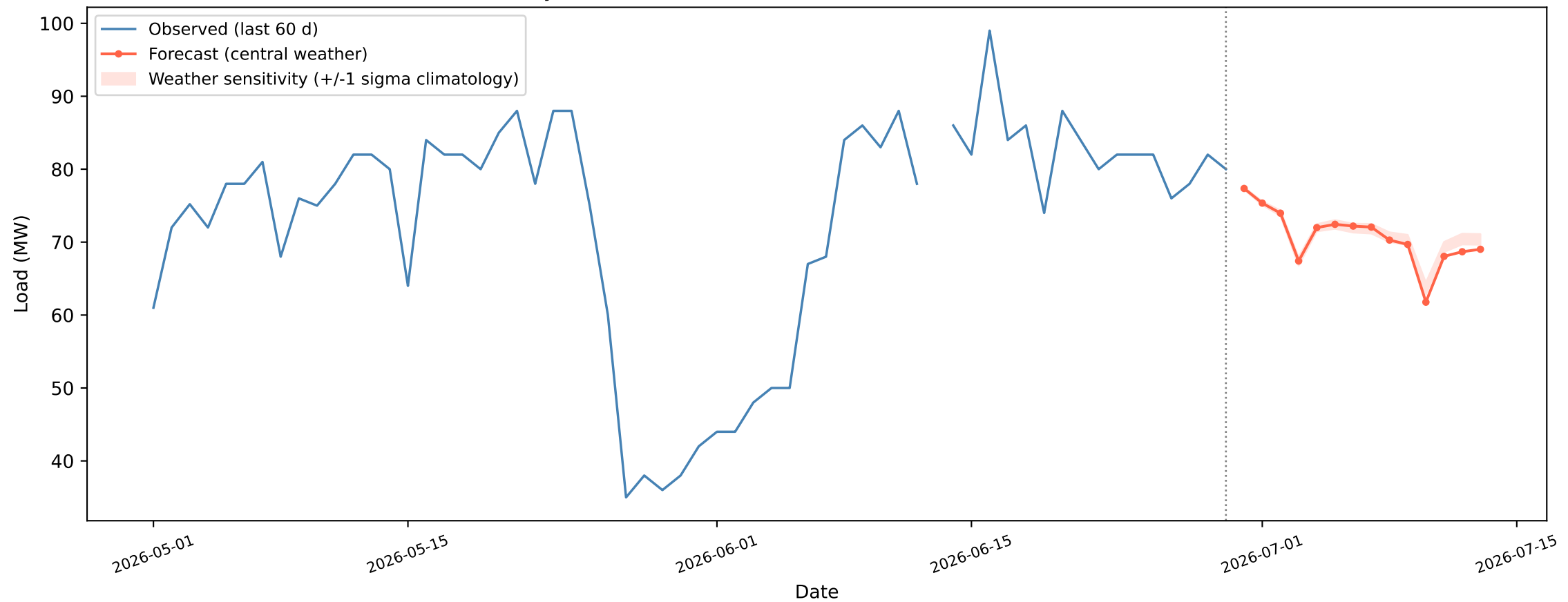
Matual - 14-day recursive forecast (BiGRU+BiLSTM), weather mode = forecast
