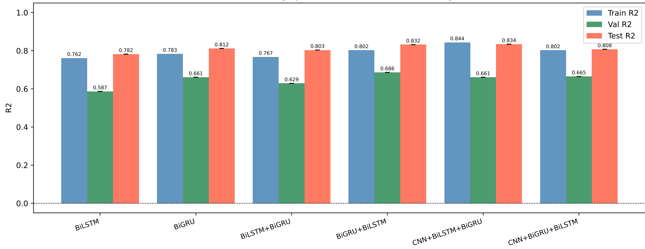
Matual - R2 by split (model selection uses VAL only)
