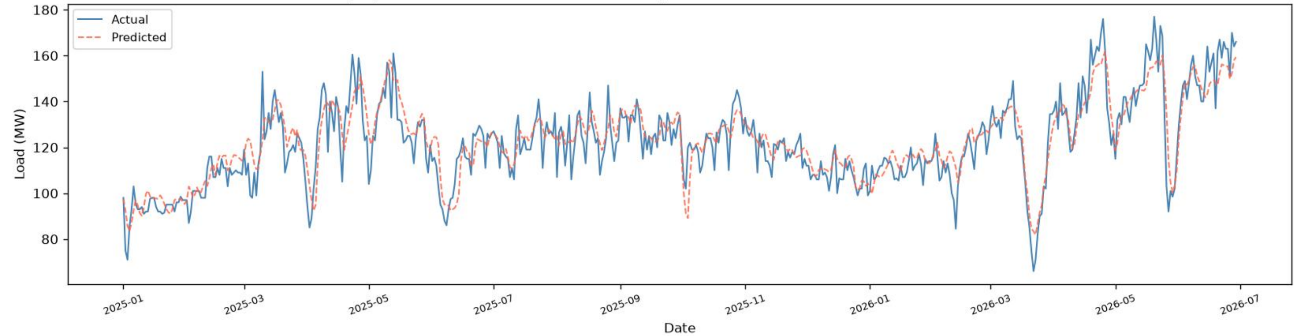
Mirpur | BiGRU+BiLSTM - TEST ( \geq 2025 ), one-day-ahead ( R^2=0.7973 , RMSE=8.47 , MAE=6.50 , n=528 )
