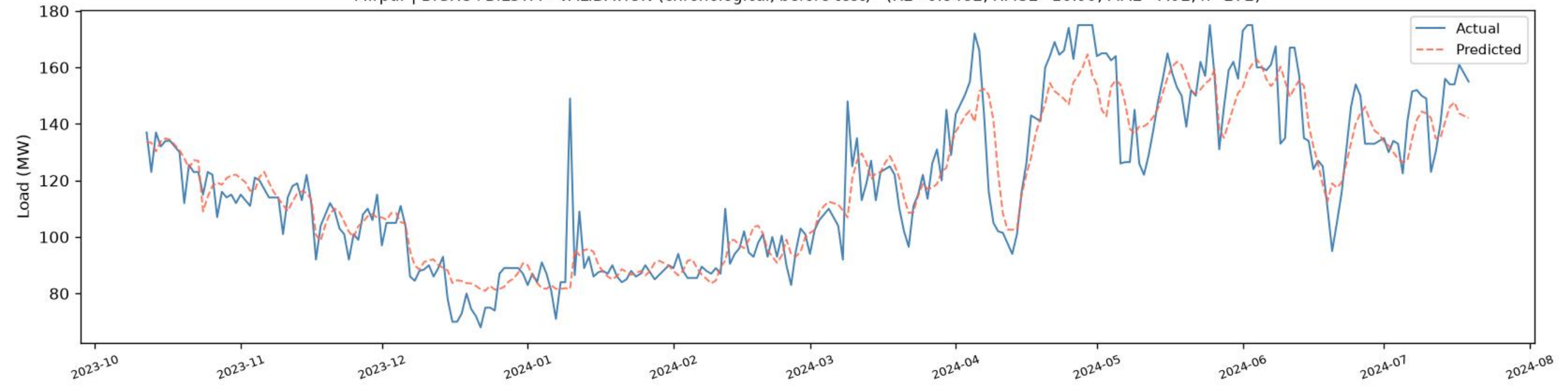
Mirpur | BiGRU+BiLSTM - VALIDATION (chronological, before test) ( R^2=0.8482 , RMSE=10.99 , MAE=7.92 , n=272 )
