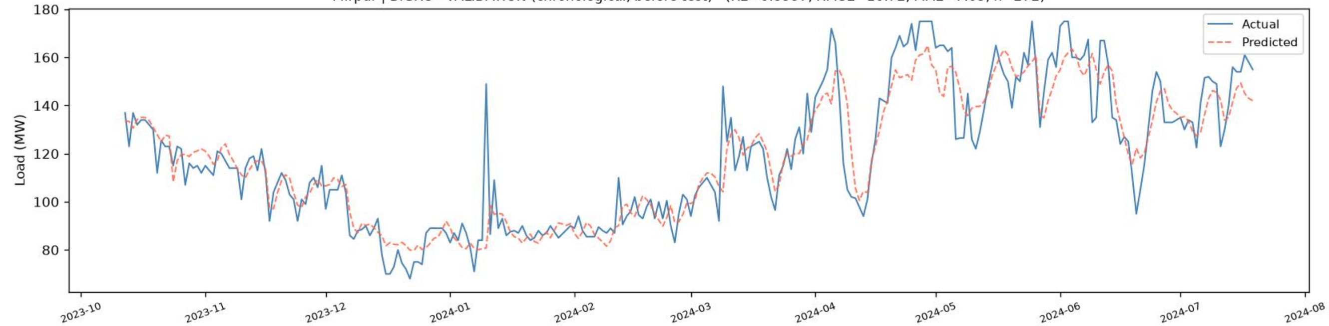
Mirpur | BiGRU - VALIDATION (chronological, before test) ( R^2=0.8557 , RMSE=10.72 , MAE=7.65 , n=272 )
