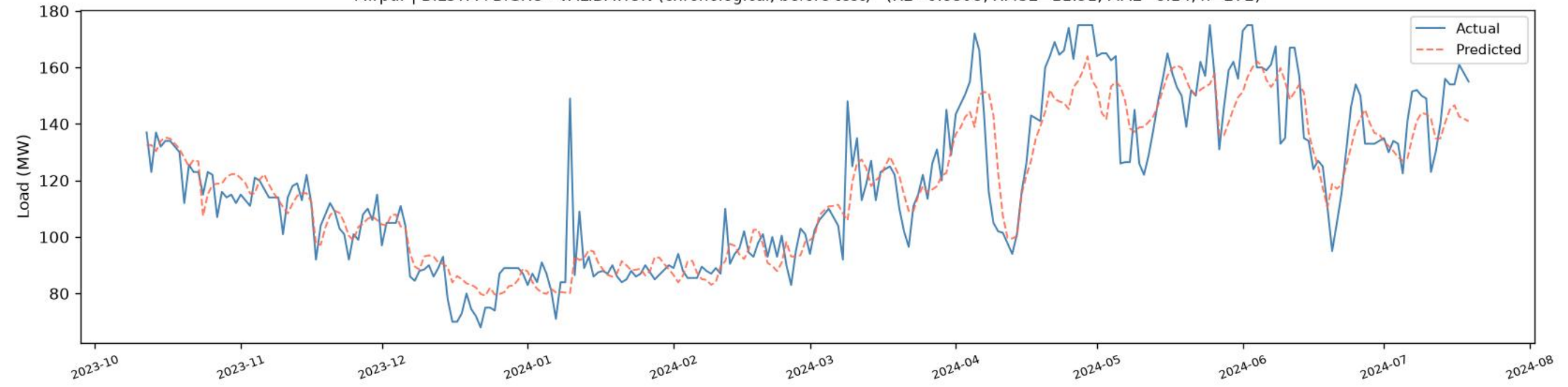
Mirpur | BiLSTM+BiGRU - VALIDATION (chronological, before test) ( R^2=0.8393 , RMSE=11.31 , MAE=8.14 , n=272 )
